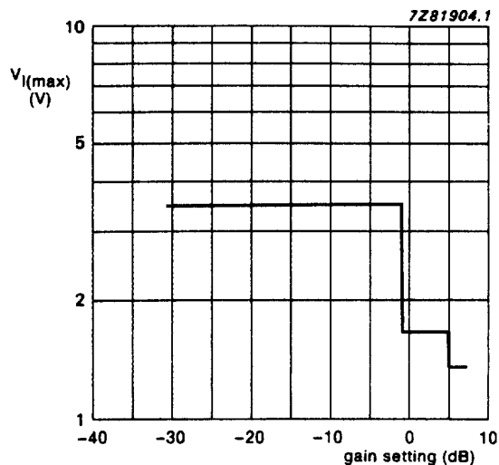
Fig.9 Input signal handling capability plotted against gain setting; THD = -60 dB; f = 1 kHz; R_S = 600 \Omega ; R_L = 10 \text{ k}\Omega ; bass/treble = 0 dB; V_{CC} = 12 V.
