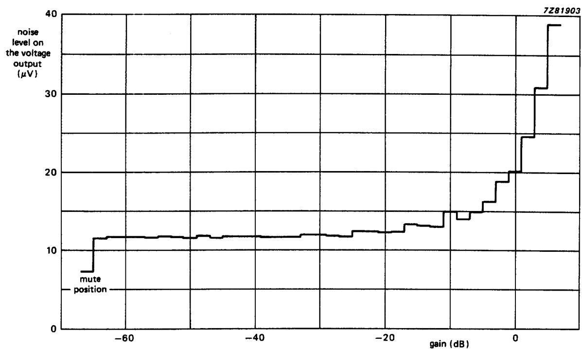
Fig.14 Noise output voltage as a function of gain; weighted CCIR 468 quasi peak gain, +6 dB to -64 dB; V_i = 0 \text{ V} ; R_S = 0 \text{ } \Omega ; R_L = 10 \text{ k}\Omega ; bass/treble = 0 dB; V_{CC} = 12 \text{ V} .
