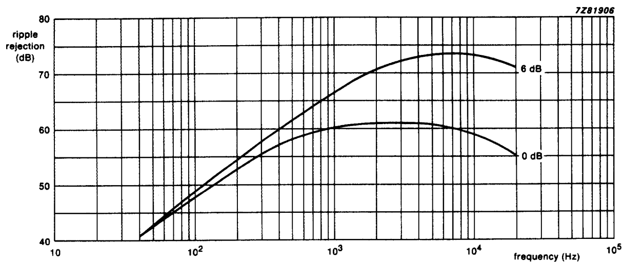
Fig.13 Ripple rejection as a function of frequency; V_{\text{ripple}} = 0.3 \text{ V (RMS)} ; R_S = 0 \text{ } \Omega ; R_L = 10 \text{ k}\Omega ; bass/treble = 0 dB; V_{CC} = 12 \text{ V} .
