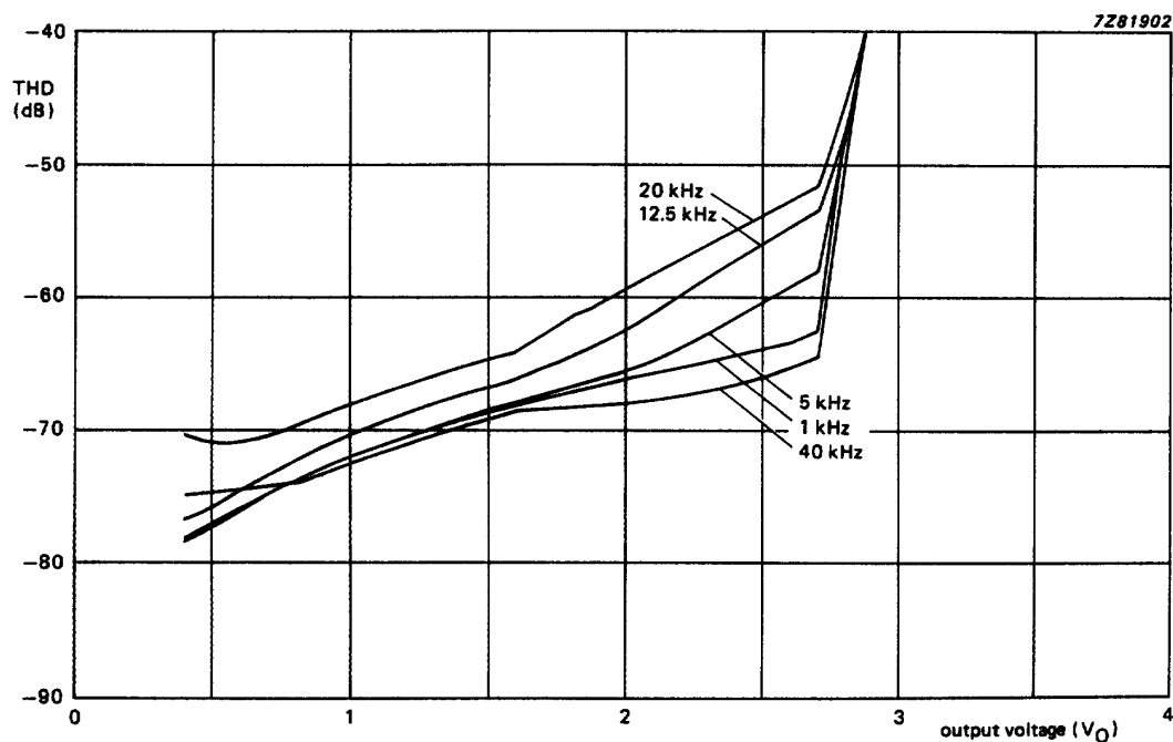
Fig.10 Output signal handling capability; gain = 6 dB; R_S = 600 \Omega ; R_L = 10 \text{ k}\Omega ; bass/treble = 0 dB; V_{CC} = 12 V.
